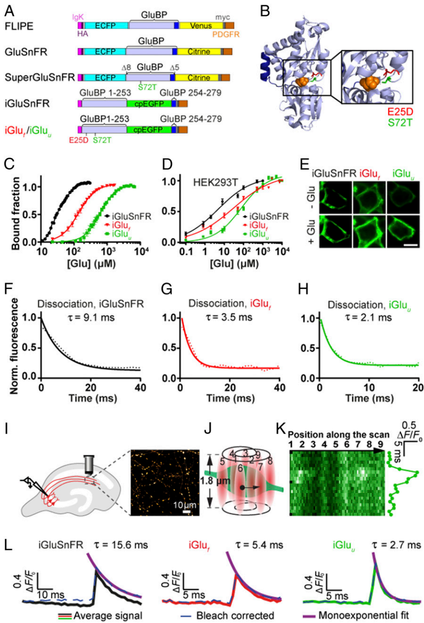
Fig. 1. Genetically encoded glutamate indicators (GEGI). (A) Domain structure and design of FRET- and single fluorophore-based GEGI; key: GluBP (blue), cpEGFP (green), IgG kappa secretion tag (pink), hemagglutinin (HA) tag (purple), myc tag (gray), and a PDGFR transmembrane domain (brown); GluBP 1–253 and 254–279 fragments are in light and dark blue, respectively; \Delta 8 aa and \Delta 5 aa specify deletions at the N and C terminus of GluBP introduced in GluSnFR. (B) Design of selected iGluSnFR variants. Crystal structure of GluBP (PDB ID code 2VHA, adapted from ref. 8). Selected mutated residues around the glutamate site are shown as red and green backbone. Bound glutamate is represented in orange space filling display. (C) Equilibrium glutamate binding titrations at 20 °C for iGluSnFR (black circles), iGluSnFR E25D (iGlu f , red triangles), and iGluSnFR S72T (iGlu u , green squares) in vitro. (D) Glutamate titrations in situ at 37 °C. iGluSnFR, iGlu f , and iGlu u were expressed in HEK293T cells and titrated with glutamate. Data derived from iGluSnFR ( n = 19 ), iGlu f ( n = 41 ), and iGlu u ( n = 33 ). (E) Representative images of HEK293T cells before glutamate addition and at saturating (1, 3, and 10 mM, respectively) glutamate. (Scale bar: 10 \mu m.) Glutamate dissociation kinetics of iGluSnFR (F), iGlu f (G), and iGlu u (H) determined by stopped-flow fluorimetry. Experimental data (dotted lines) are overlaid by curves fitted to single exponentials (solid lines). Fluorescence changes are normalized to F_{max} of 1. Imaging glutamate release from single presynaptic terminals. (I) Schematic representation of hippocampal slice with transfected and patch-clamped CA3 pyramidal cell. (J) Spiral scan intersecting site of vesicular fusion. (K) Zoomed-in image of single trial iGlu u response. (L) Decay time ( \tau_{off} ) measurements with bleach correction (dashed lines) for individual experiments by single exponential fit for iGluSnFR ( n = 13 boutons, 500 Hz sampling rate) and variants iGlu f ( n = 7 boutons, 1 kHz sampling rate) and iGlu u ( n = 7 boutons, 1 kHz sampling rate).
